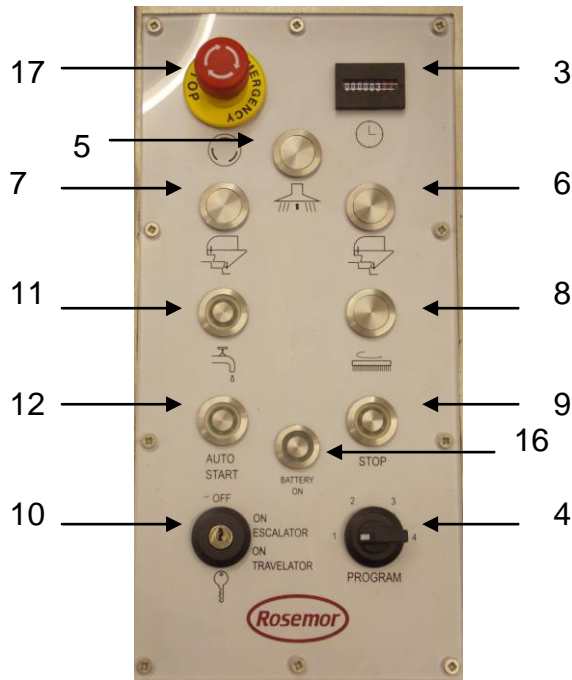
Fig. 2: Control Panel
